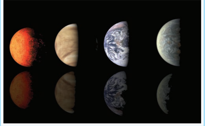
NASA/Ames/JPL-Caltech
